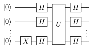
■ Figure 8 The Deutsch-Jozsa algorithm in SQIR and as a circuit. The Coq function npar constructs a SQIR program that applies the same operation to every qubit.
